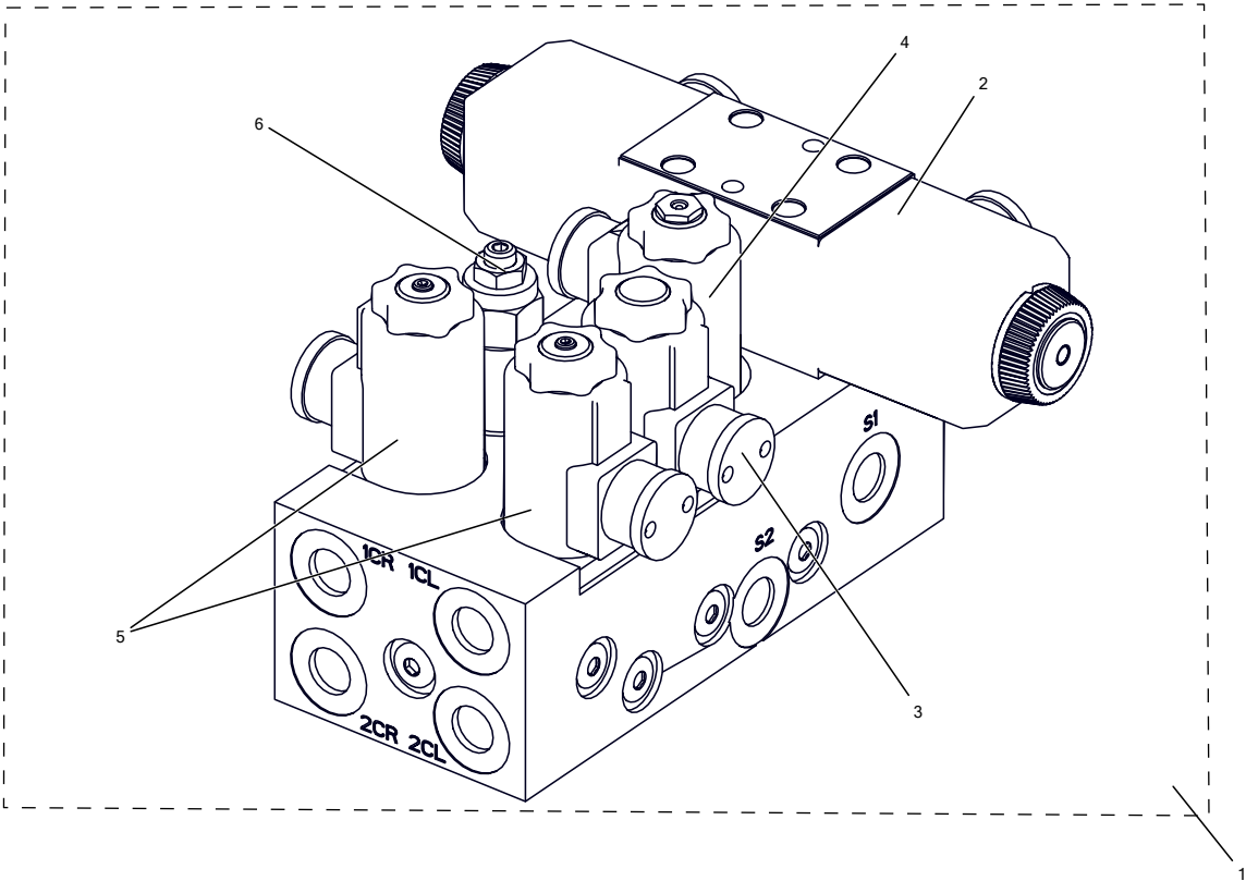
Figure 43: YBLOCK5 ARRANGEMENT
