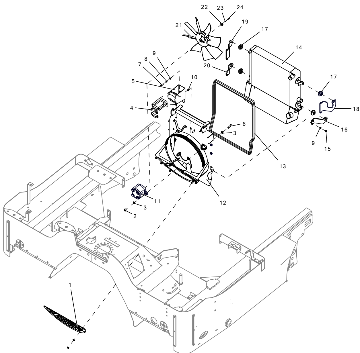
Figure 206: LM1-106-220 HATZ ENGINE COOLING SYSTEM FAN ASSEMBLY
