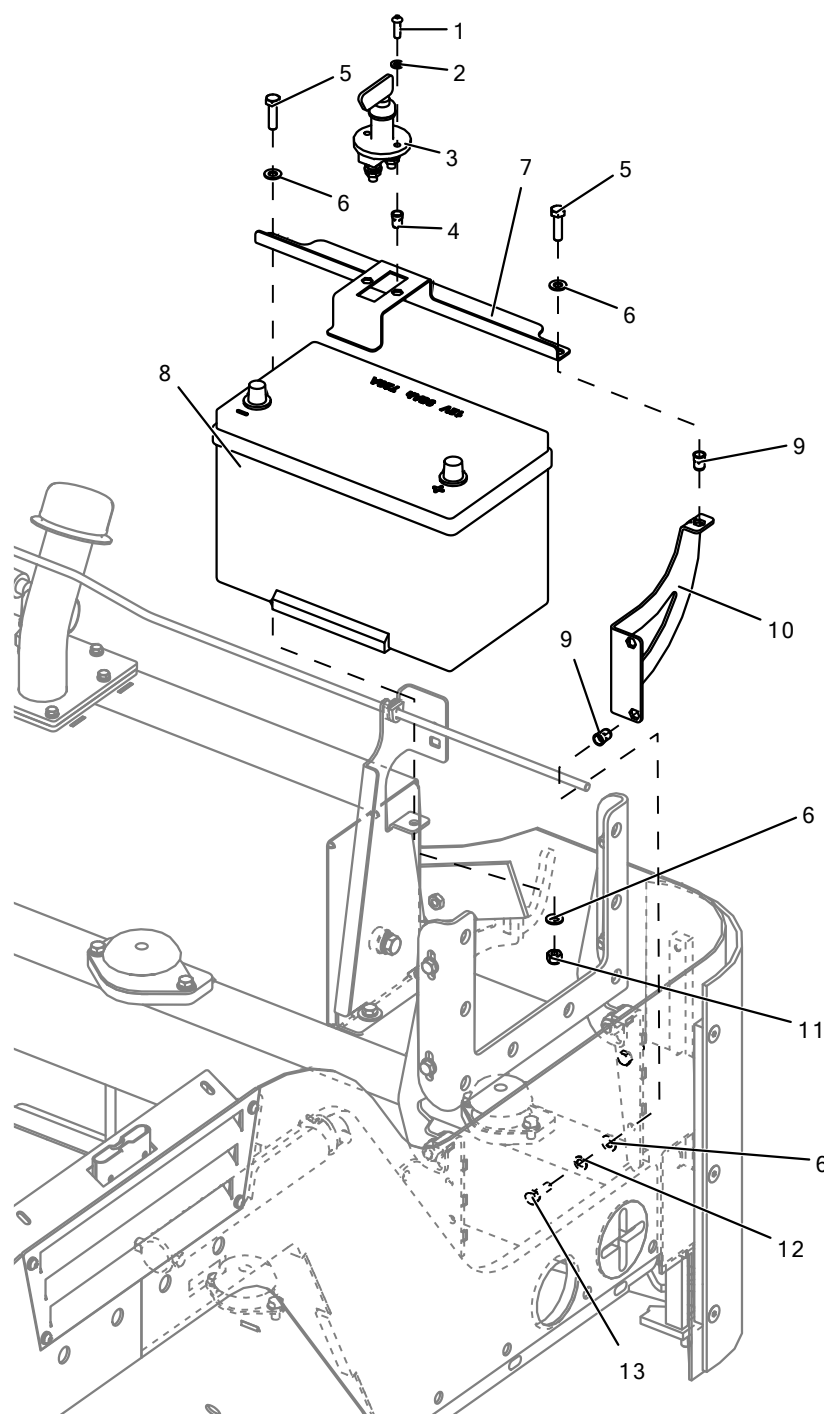
Figure 14: LM1-870-10 BATTERY AND MOUNTING ASSEMBLY
