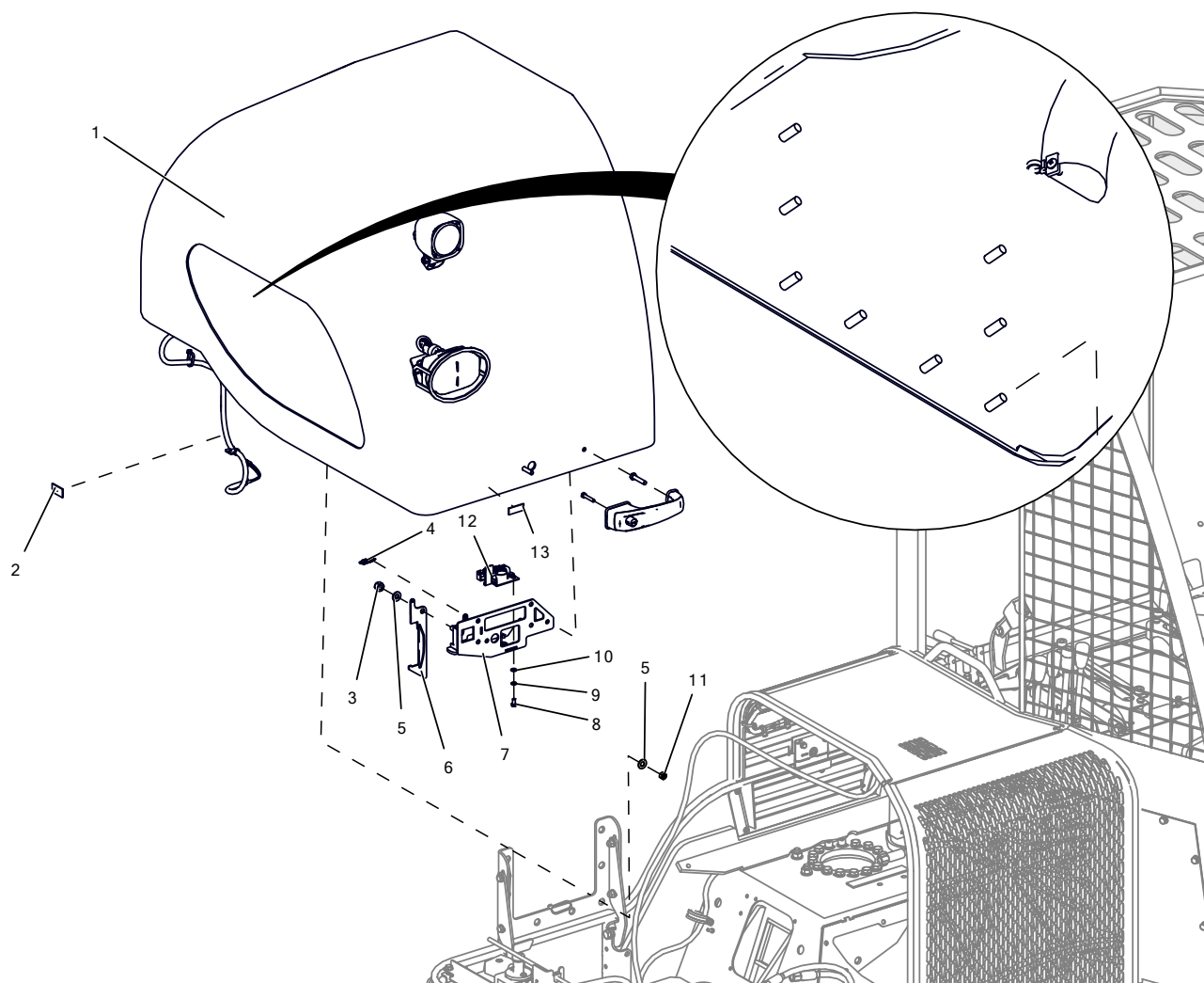
Figure 59: LM1-125-85 BONNET ASSEMBLY TO CHASSIS
