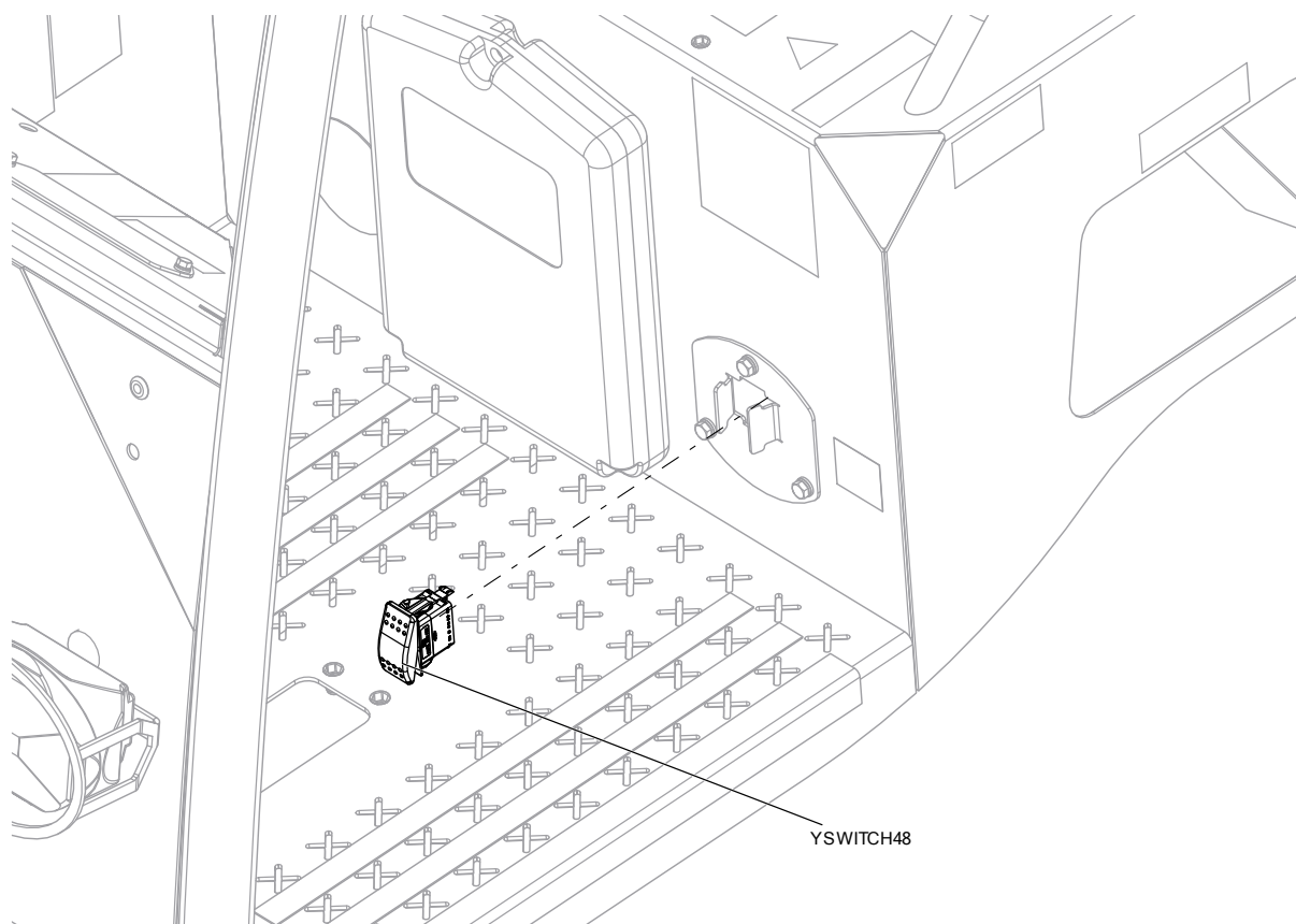
Figure 156: LM1-500-500 YSWITCH48 DUMP VALVE SWITCH
