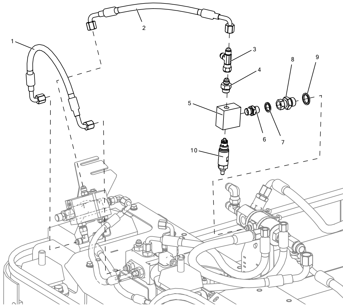
Figure 45: LM1-720-82 400BAR ISR RELIEF VALVE JIC ASSEMBLY
