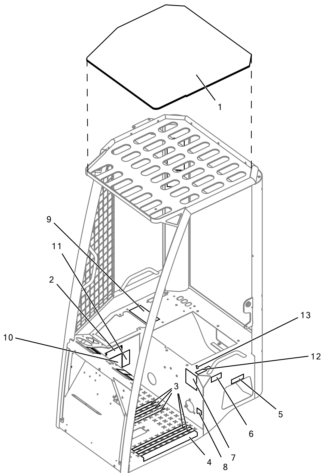
Figure 152: LM1-501-97 CAB FRAME WITH ROOF AND DECALS
