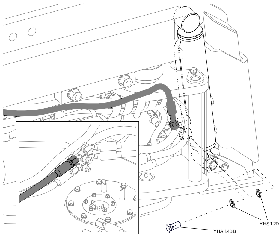
Figure 109: JIC - LM1-350-10 STABILISER LEG LHS TOP PORT 4 WAY CONFIGURATION
