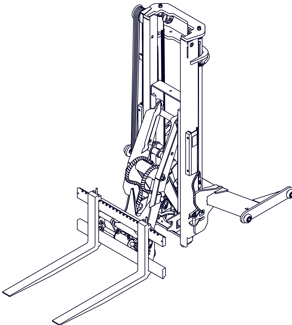
Figure 122: LM1-21-10 3.6M MAST ASSEMBLY
