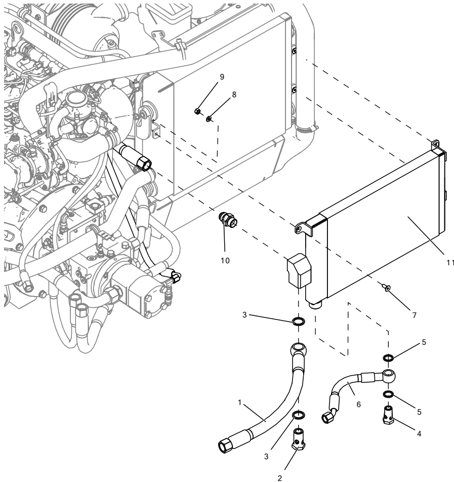
Figure 213: LM1-106-222 OIL COOLER DETAIL
