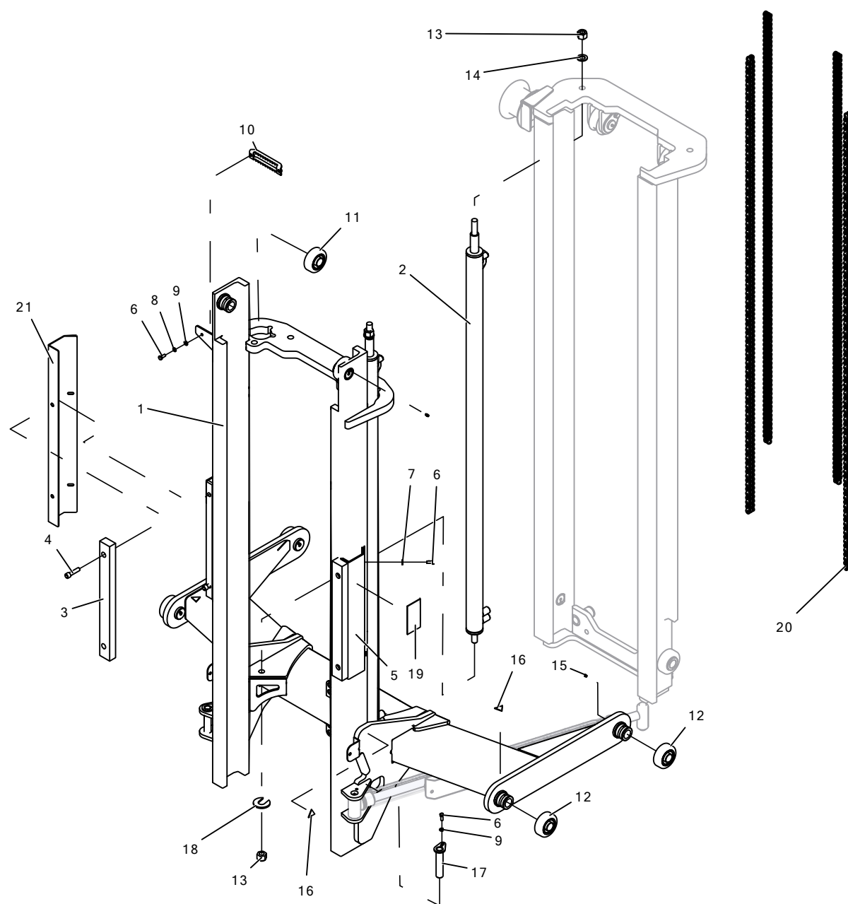
Figure 123: LM1-232-50 STAGE 1 MAST 3.6M
