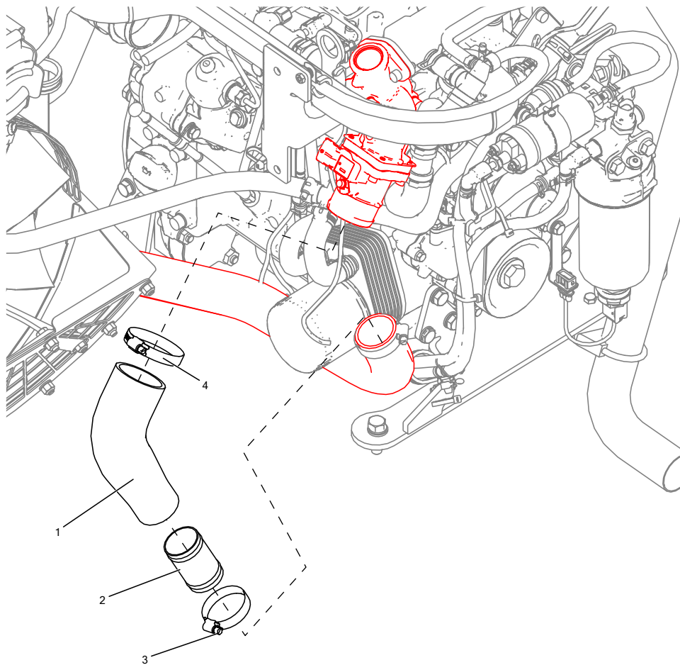
Figure 204: LM1-600-60 INTAKE RUNNER ADAPTER
