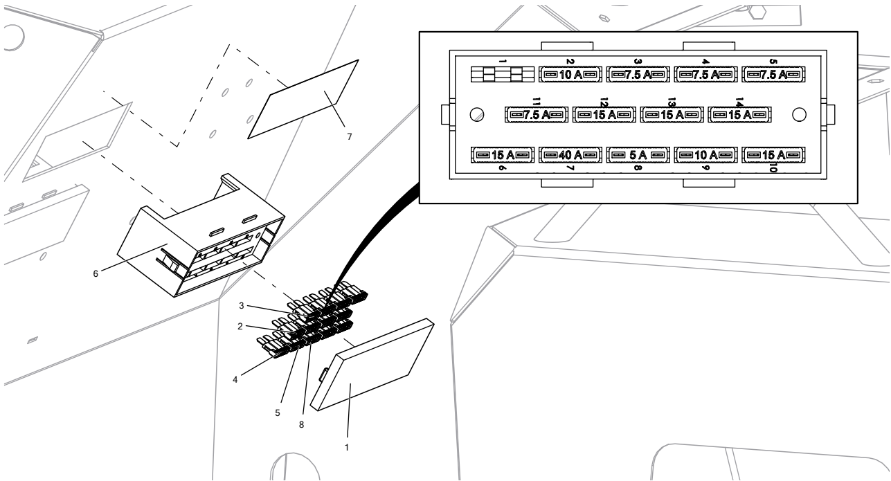
Figure 168: LM1-840-04 YFUSEBOX2 FUSES STANDARD ACCESSORIES – 2 WAY
