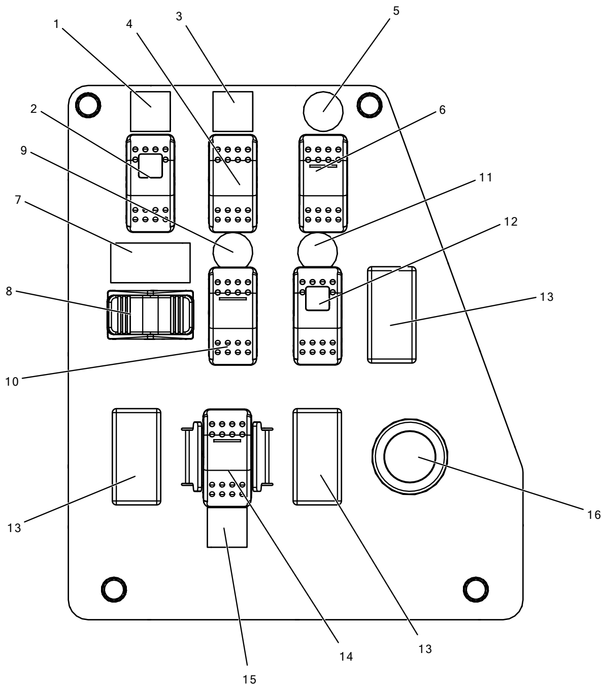
Figure 177: LM1-516-50 MAIN SWITCH PANEL AUS 2-WAY
