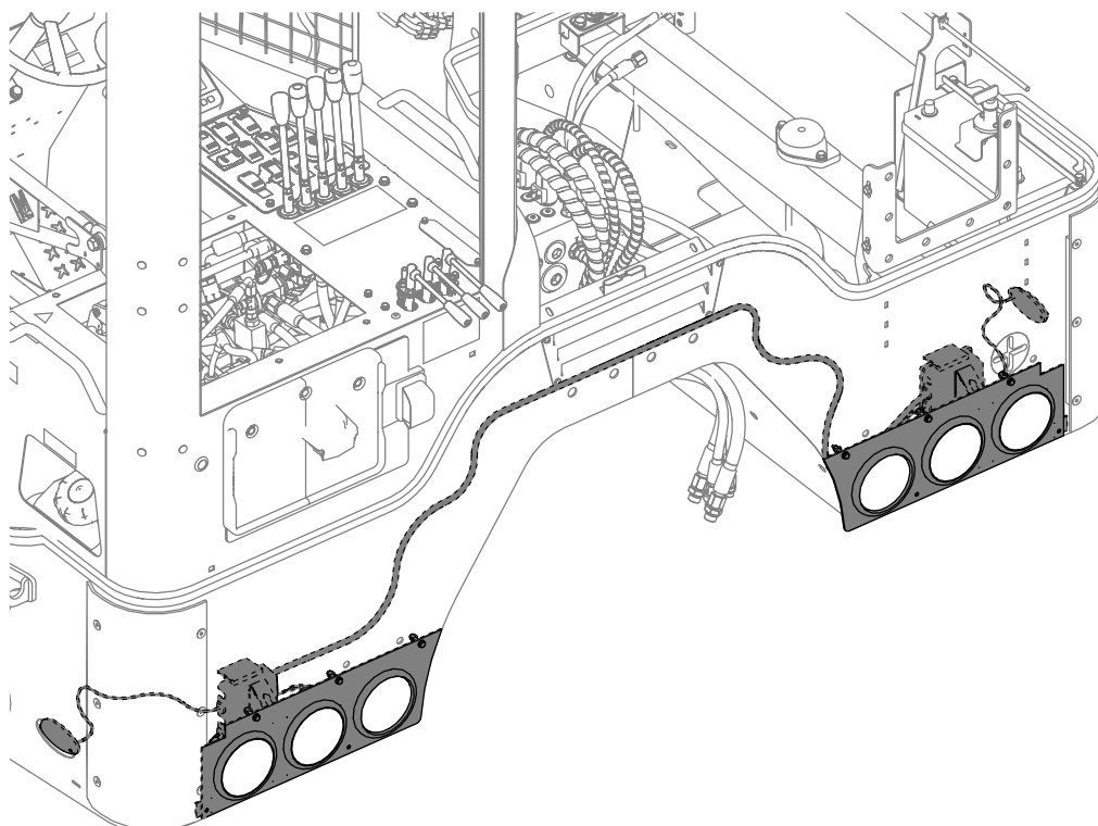
Figure 50: Chassis lights general layout
