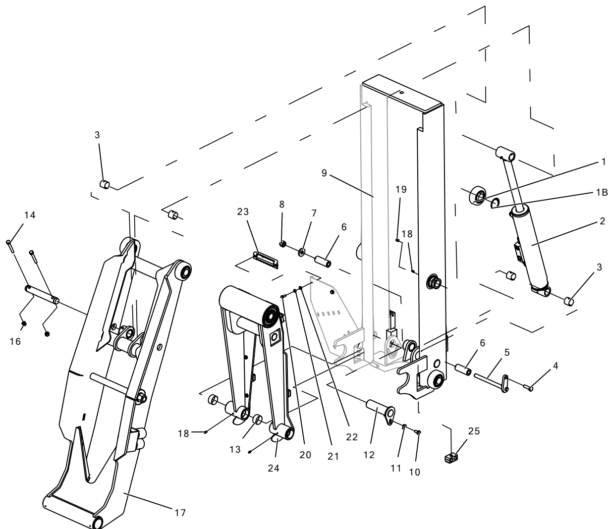
Figure 129: LM1-24-00 3RD STAGE BODY TO ISR PARTS
