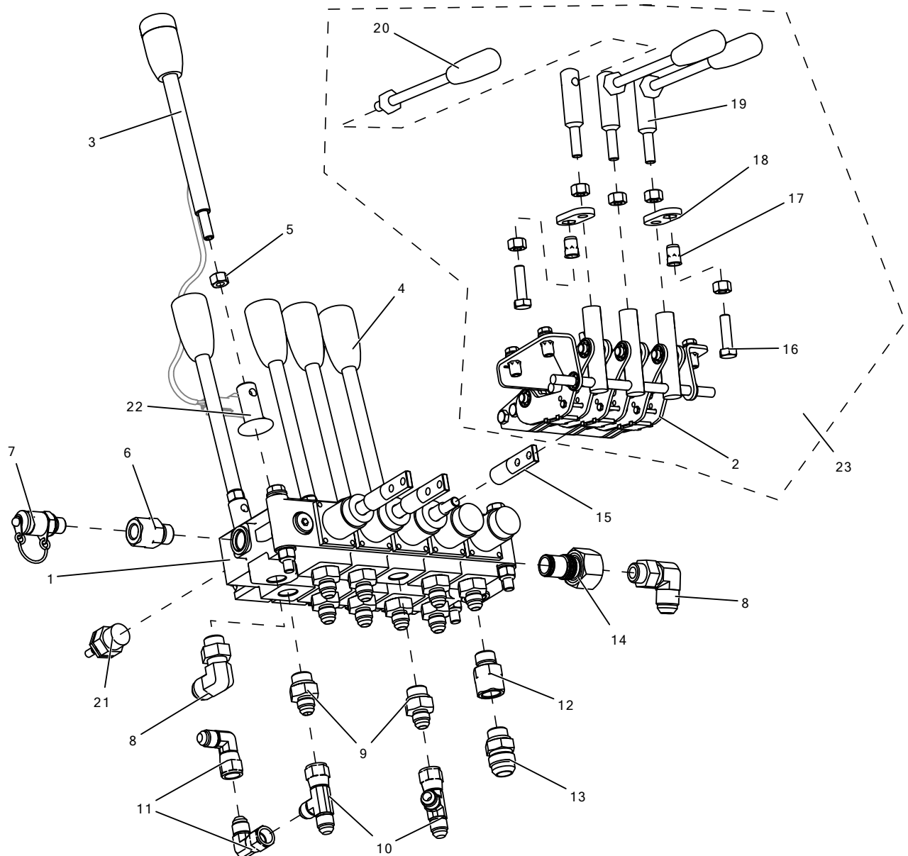
Figure 181: LM1-730-02 JIC LEVER CONTROL STANDARD
