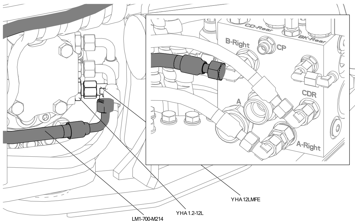
Figure 101: LM1-702-30 METRIC RHS FRONT HYDRAULICS LM1-700-M214 TO YBLOCK3 [B-RIGHT] 4 WAY CONFIGURATION
