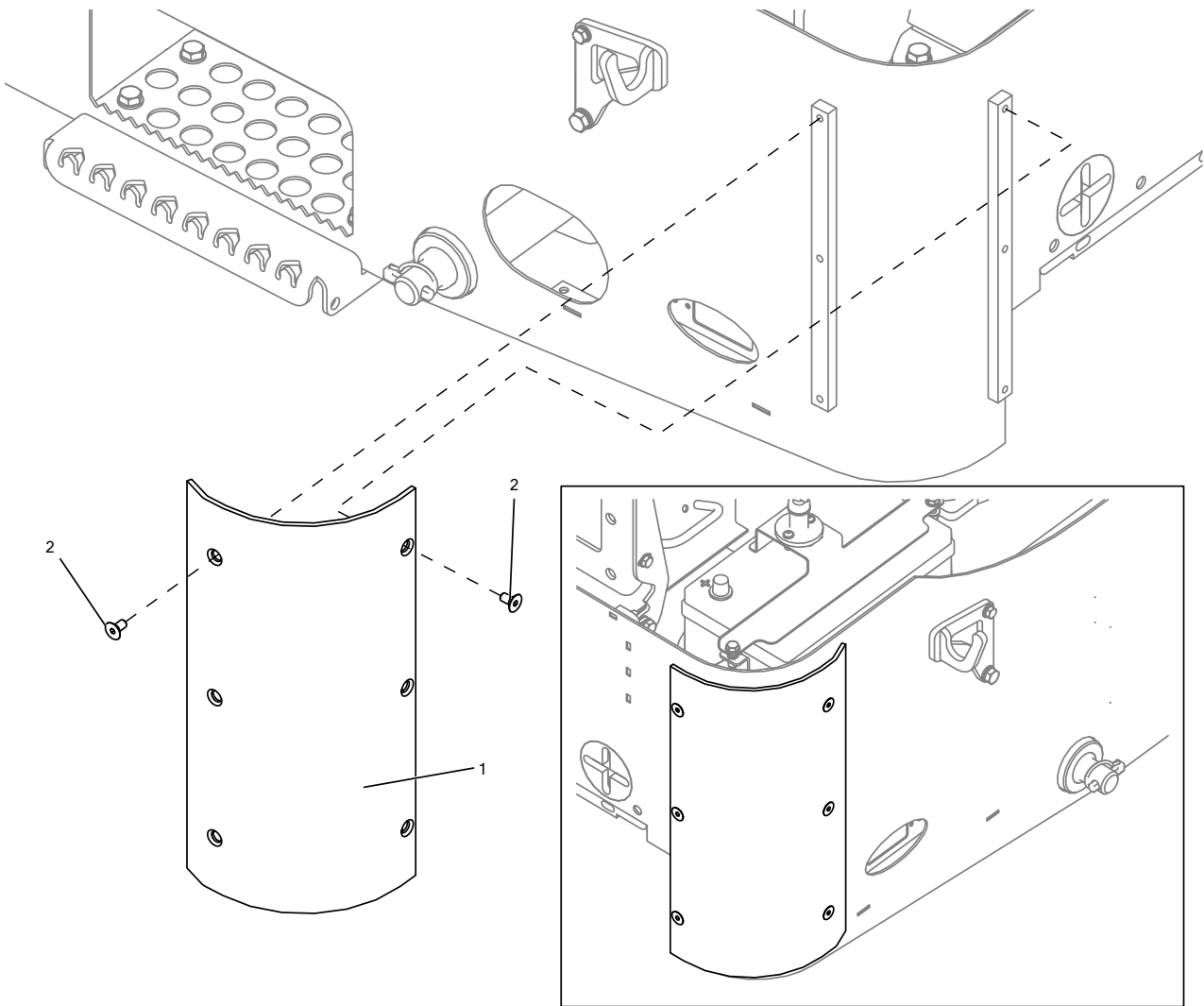
Figure 7: LM1-100-270 CORNER GUARD
