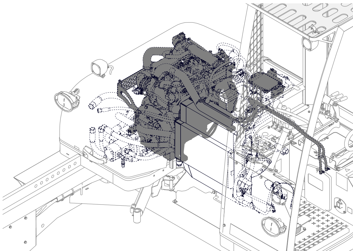
Figure 195: LM1-604-20 HATZ ENGINE TIER 4 FINAL T4F COMPLETE
