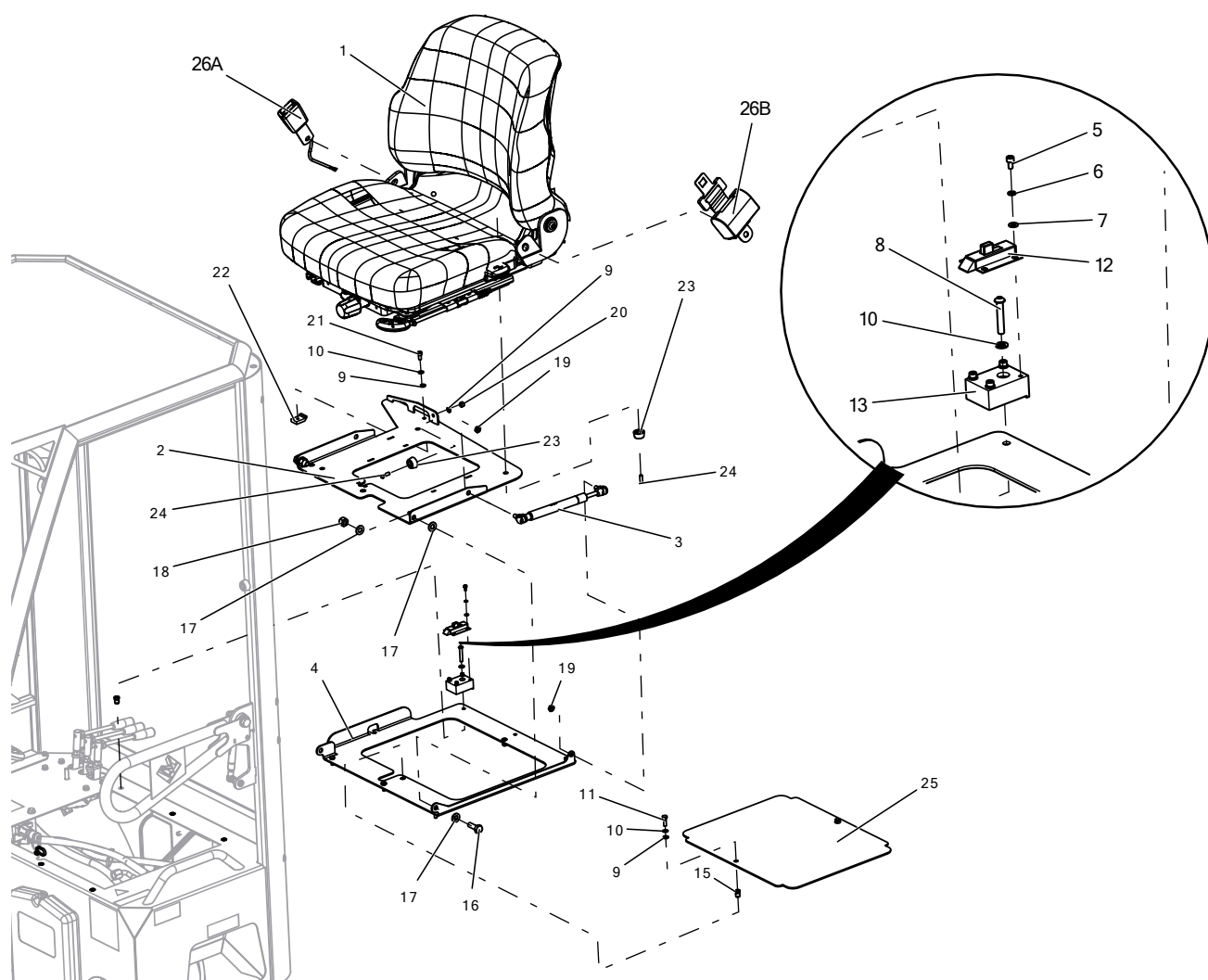
Figure 147: LM1-500-100 SUSPENSION SEAT
