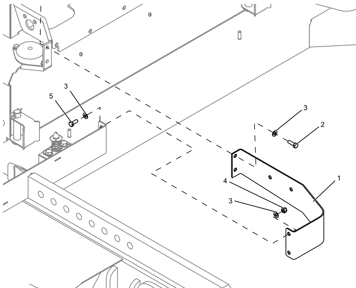
Figure 20: LM1-100-73 RH VALANCE
