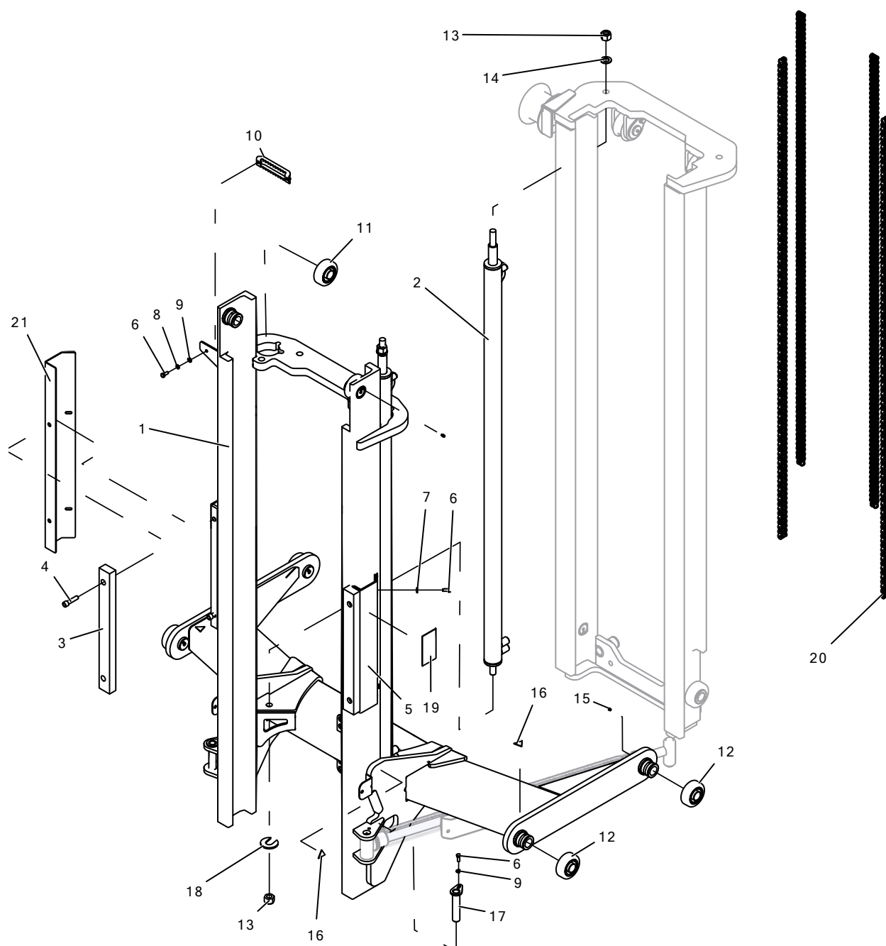
Figure 118: LM1-202-50 STAGE 1 MAST 3.1M
