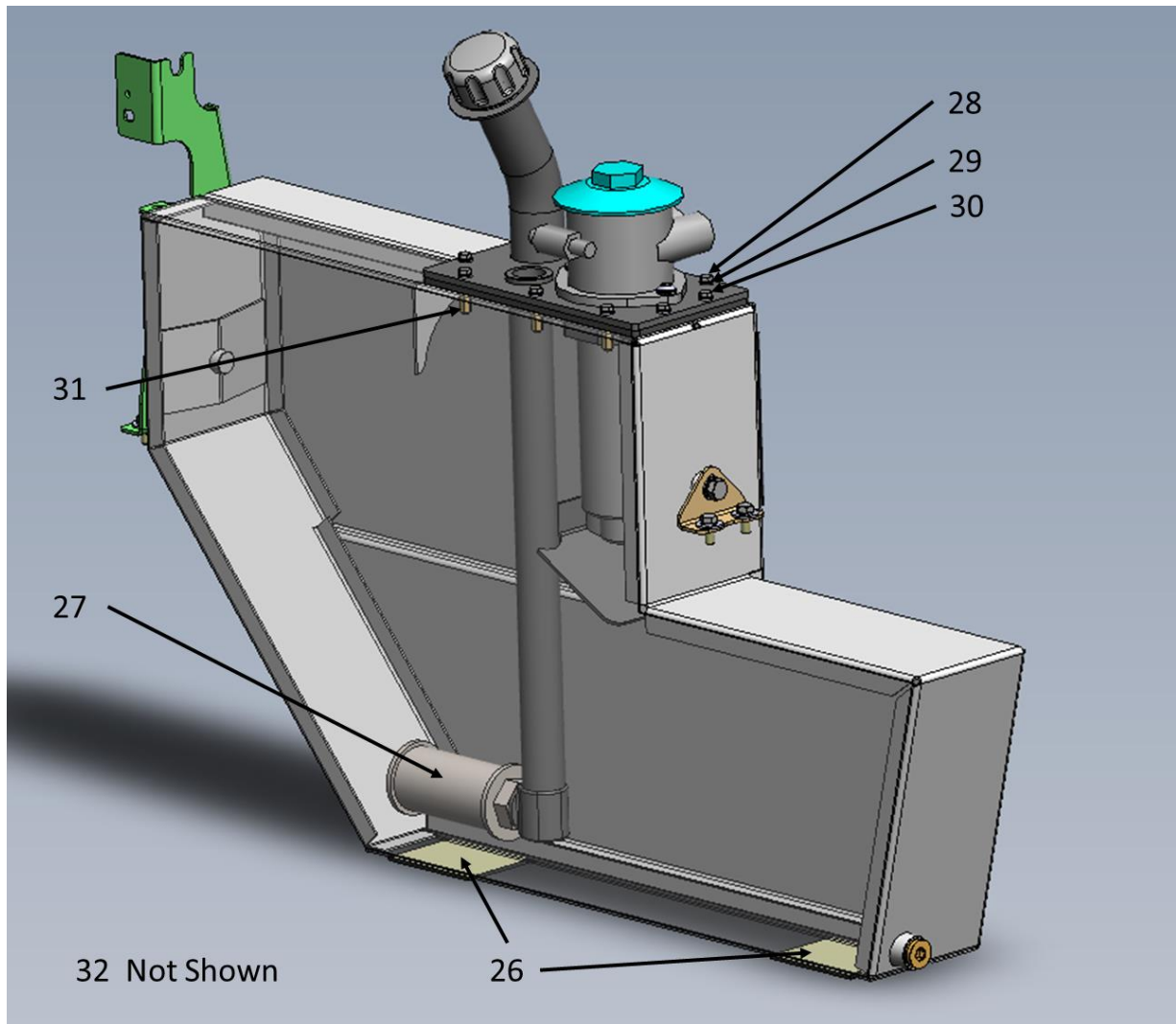
Figure 3: 855 Drop in Hydraulic Internal parts – S.N. 855-500 to date
