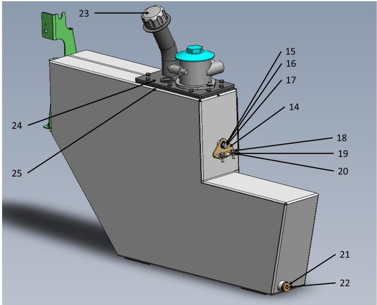
Figure 2: 855 Drop in Hydraulic Tank – S.N. 855-500 to date
