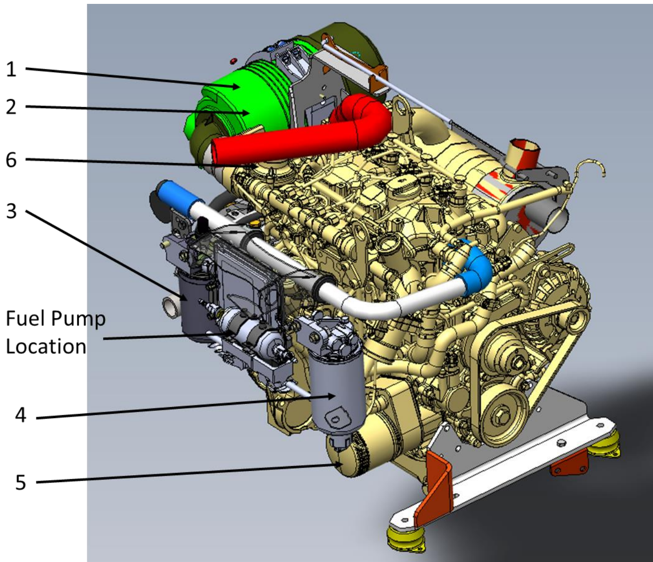
Figure 1: Hatz Engine Layout – S.N. 855-500 to 855-712
